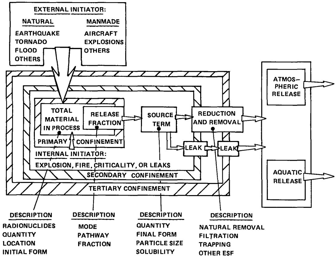
Fig. 2. Accident release steps.
